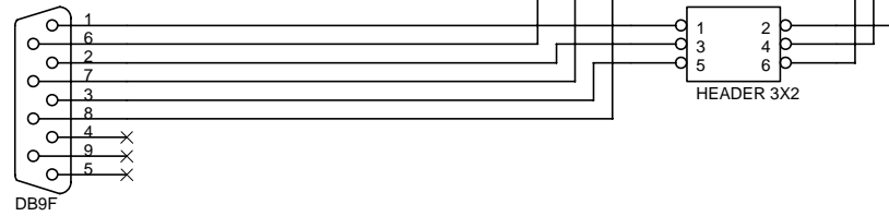
BDM CABLE - 6 PIN (STANDARD)
