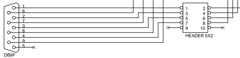
BDM CABLE - 10 PIN (+MODA,MODB)
